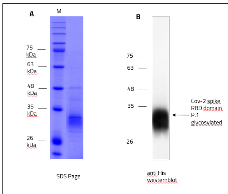
Fig. 1: Size and purity of CoV-2 spike protein P.1 RBD domain assessed by SDS-PAGE, Western Blot using a Rho1D4 antibody.
